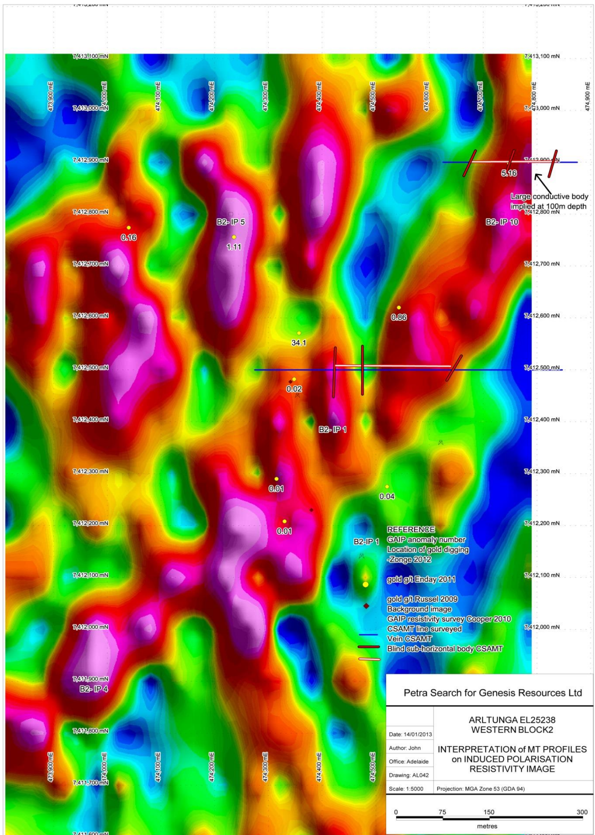
Figure 6 Location of western CSAMT profiles on GAI resistivity image
